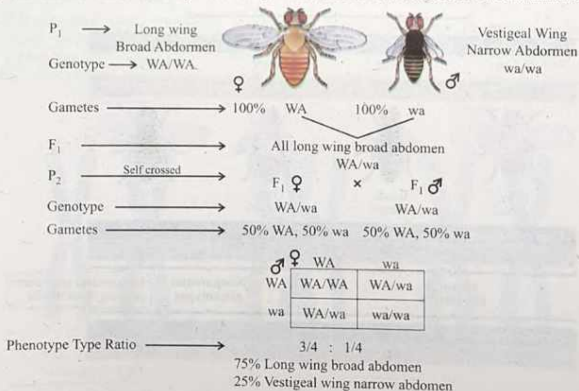
Fig.22.10: Morgan Experiment
