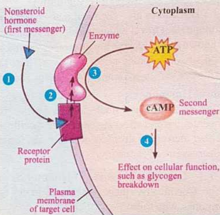
Fig. 18.1: Action of Non-steroid Hormone
