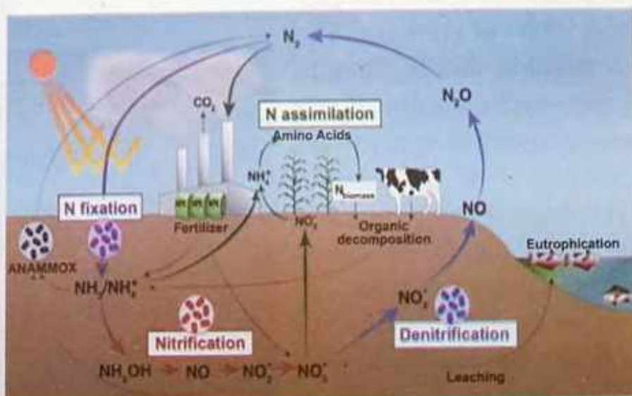
Fig. 25.3: Nitrogen Cycle
