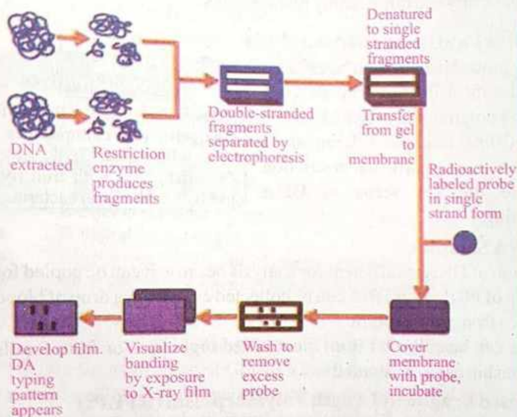
Fig. 26.10: Southern Blotting
