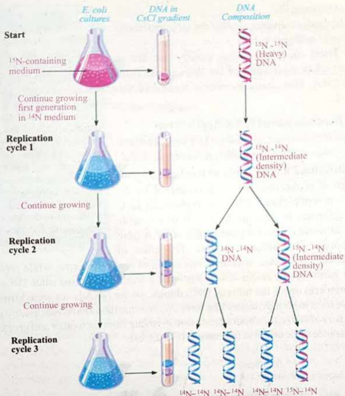
Fig. 23.12: Meselson-Stahl Experiment
