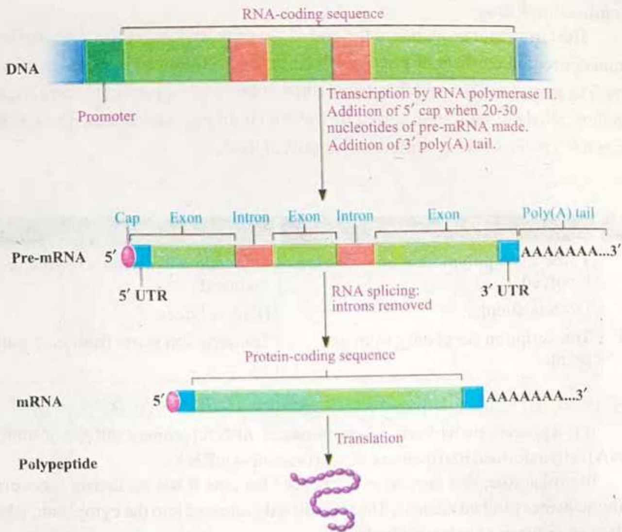
Fig. 23.19: mRNA Processing
