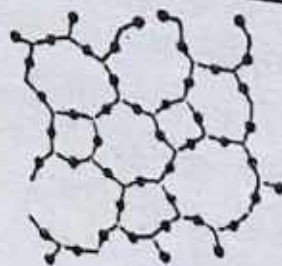
Amorphous quartz
