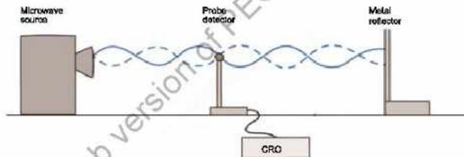
Fig. 7.10: Experimental setup for stationary waves using microwave
