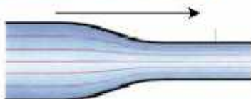
Fig. 5.11: Streamlines (laminar flow)
