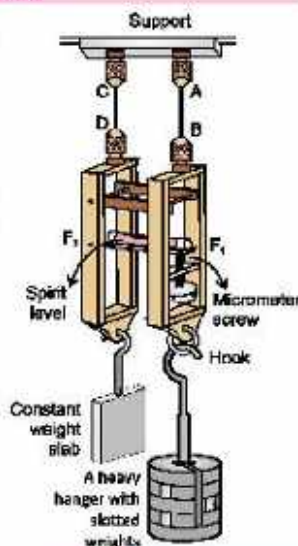
Fig. 5.4: Searle's apparatus
