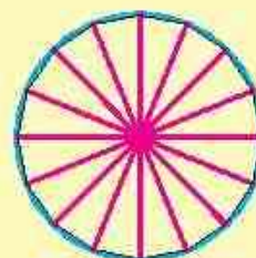
Figure 12.3: 16-sided polygon
