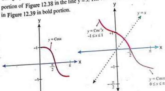
Figure 12.39 Graph of \text{Cos} x and \text{Arc Cos} x
