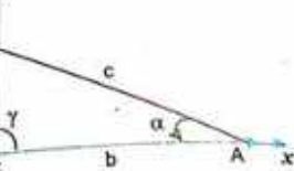
(ii) \gamma is obtuse Figure 11.12(b)
