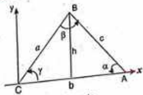
(i) \gamma is acute Figure 11.12(a)
