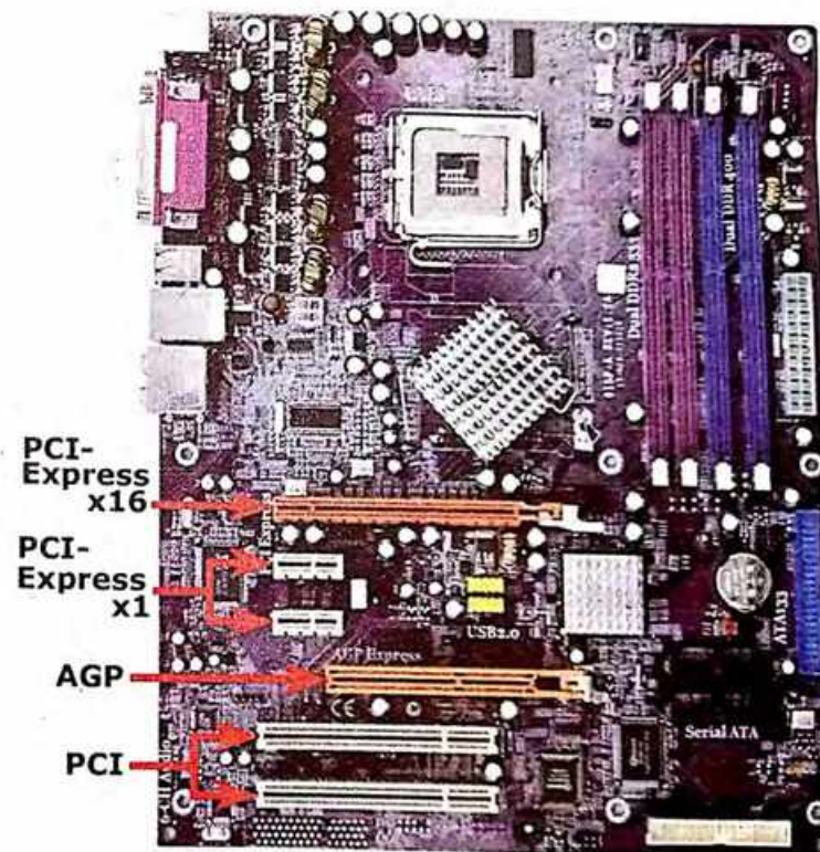
Figure 4.7 Expansion Slots
