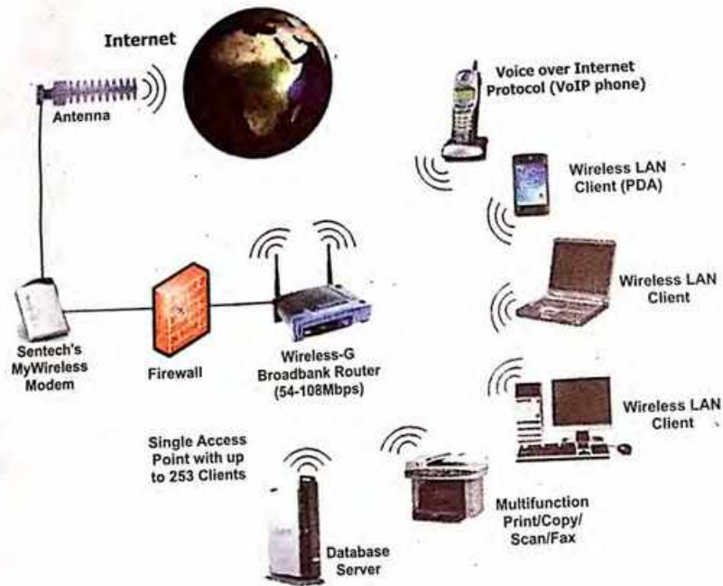
Figure 6.1 Wireless Network
