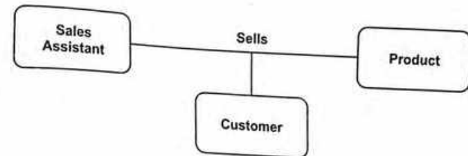
Figure 7.12 Ternary relationship
