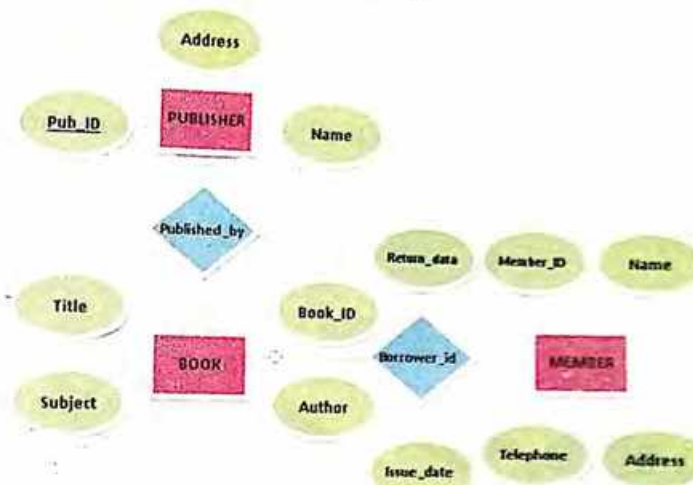
Figure 7.18 E-R Diagram for Library Management System
