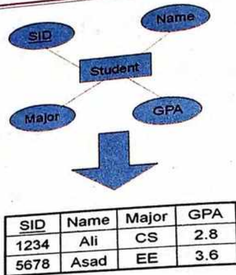
Figure 7.21 Transformation of E-R Model into Relational Schema
