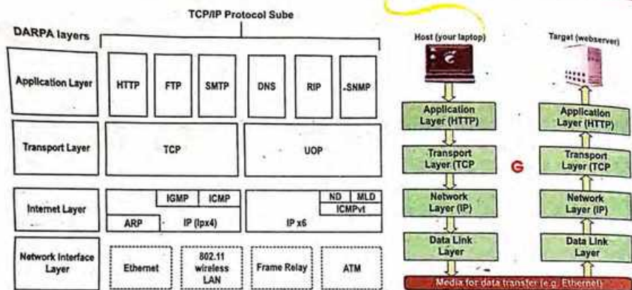
Figure 5.28 The architecture of the TCP/IP protocol suite
