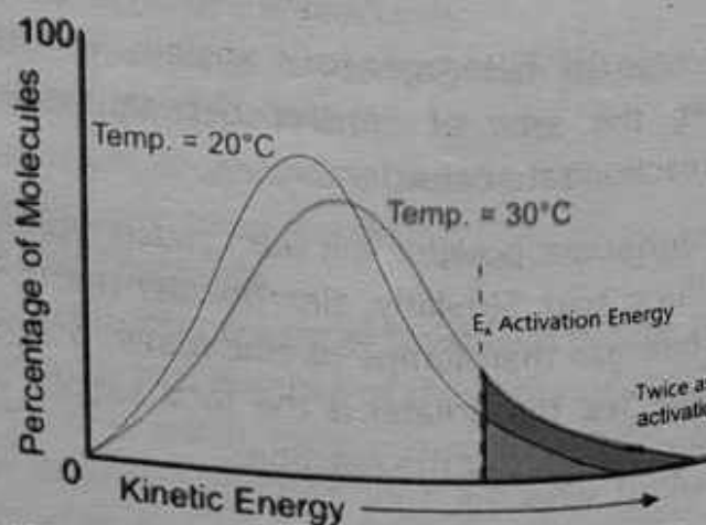
Fig: 9.3 Effect of Temperature on Rate of Reaction
