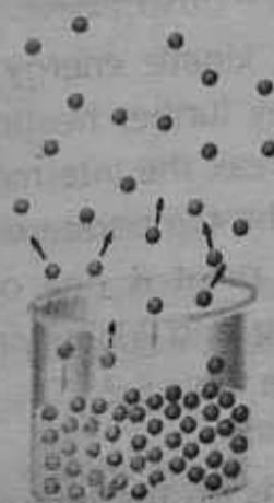
(b) Vaporization > condensation rate
