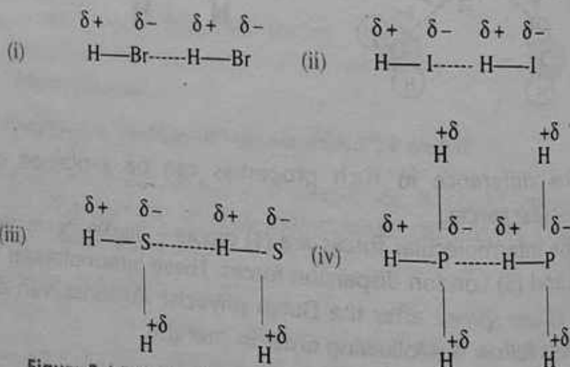
Figure 5.4 Dipole-Dipole Forces in HBr, HI, \text{H}_2\text{S} and \text{PH}_3
