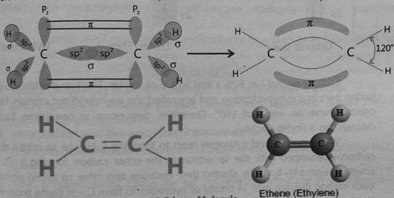
Figure 3.22 Ethene Molecule
