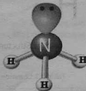
VSEPR Model of \text{NH}_3
