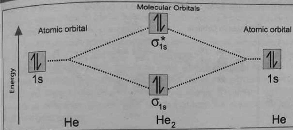
Figure 3.26 Molecular Orbital Diagram of Helium \text{He}_2 molecule
