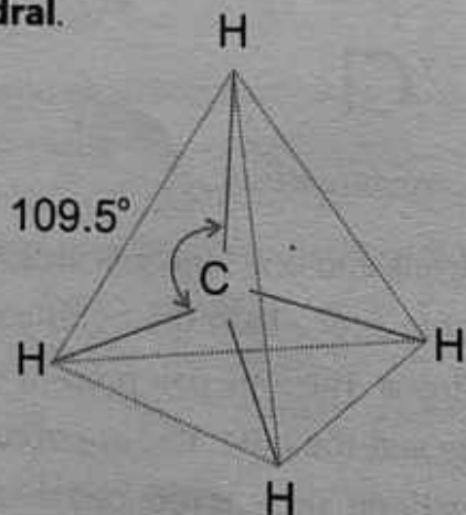
Tetrahedral Structure of \text{CH}_4
