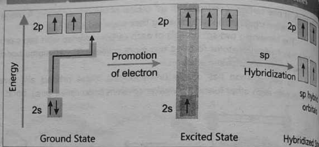
Figure 3.23 sp Hybridization
