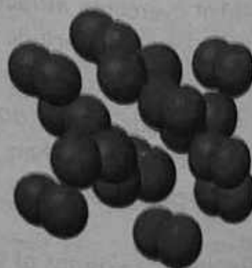
Figure 3.31 Molecular Solids of Carbon dioxide ( \text{CO}_2 ) and Iodine ( \text{I}_2 )
