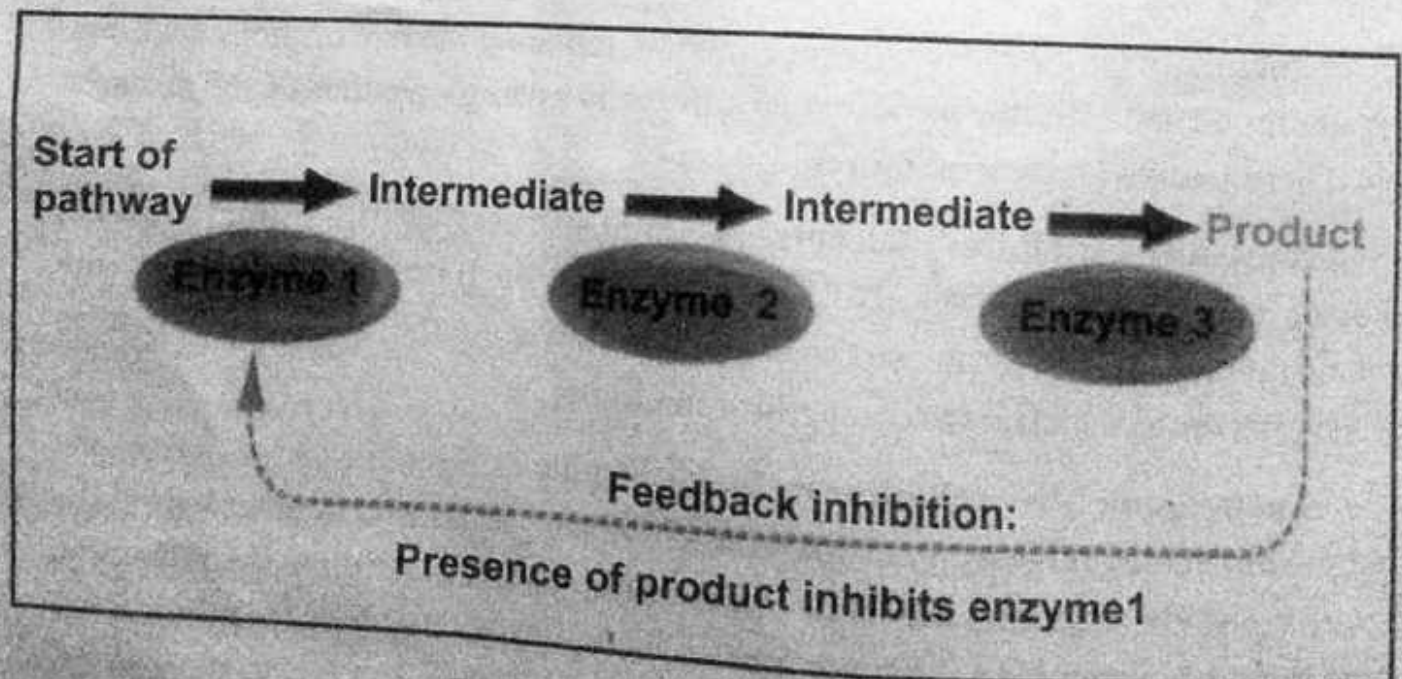
Fig. 3.6 Feedback inhibition.
