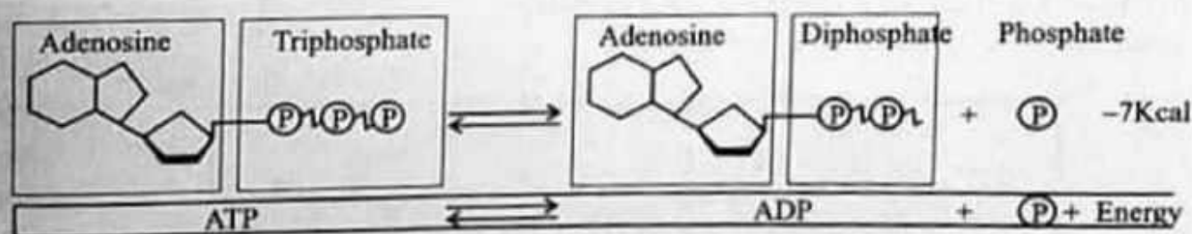
ATP Reaction
