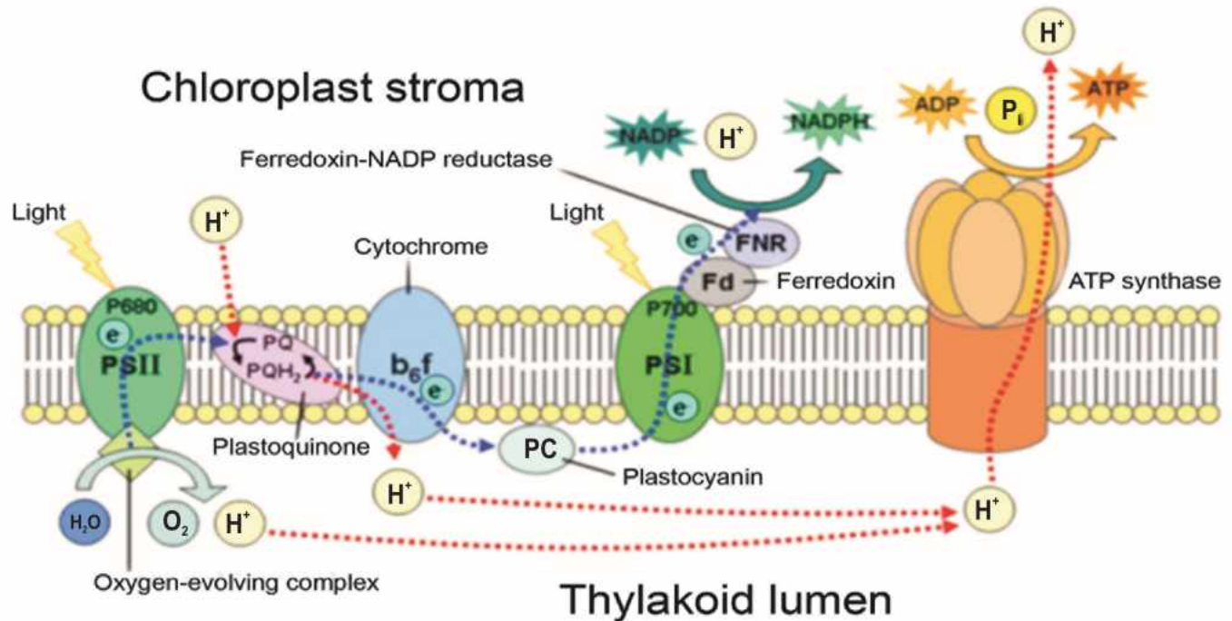
Fig. 4.7: Chemiosmotic synthesis of ATP during light reaction
