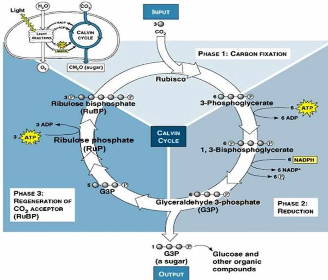
Fig 4.10: Calvin cycle
