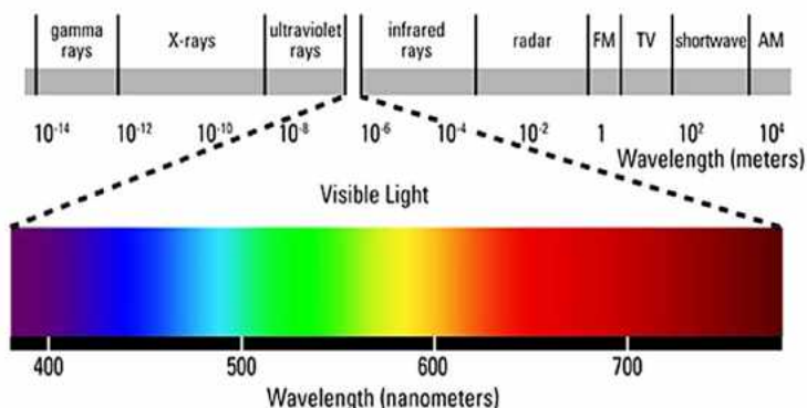
Fig. 4.1 Electromagnetic spectrum
