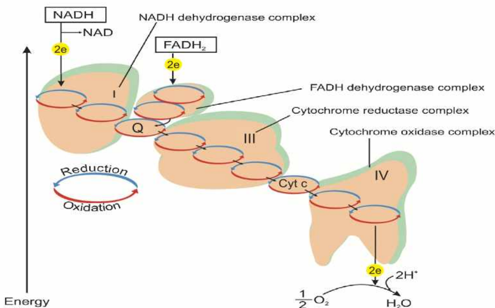
Fig: 4.17 Sequence of electron carriers in respiratory ETC
