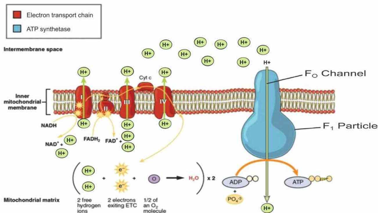
Fig. 4.18: Mechanism of chemiosmosis in respiratory electron transport chain
