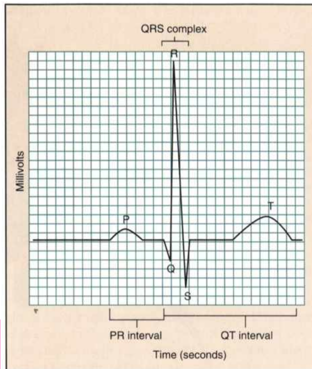
Figure 12.5 Electrocardiogram (ECG)
