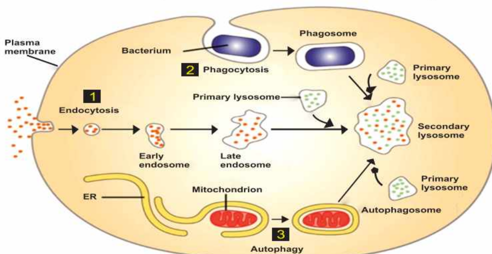
Fig. 1.19: Functions of Lysosomes
