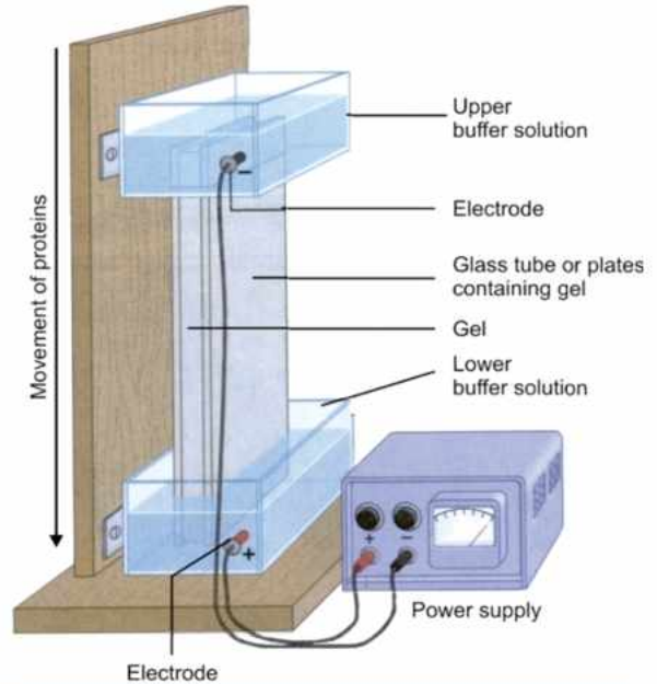
Fig. 1.4: Gel electrophoresis
