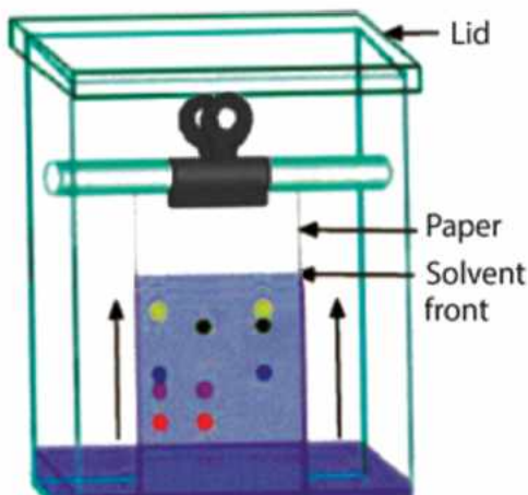
Fig. 1.3: Chromatography chamber
