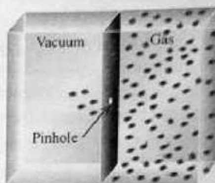
Figure 4.10(b): Effusion
