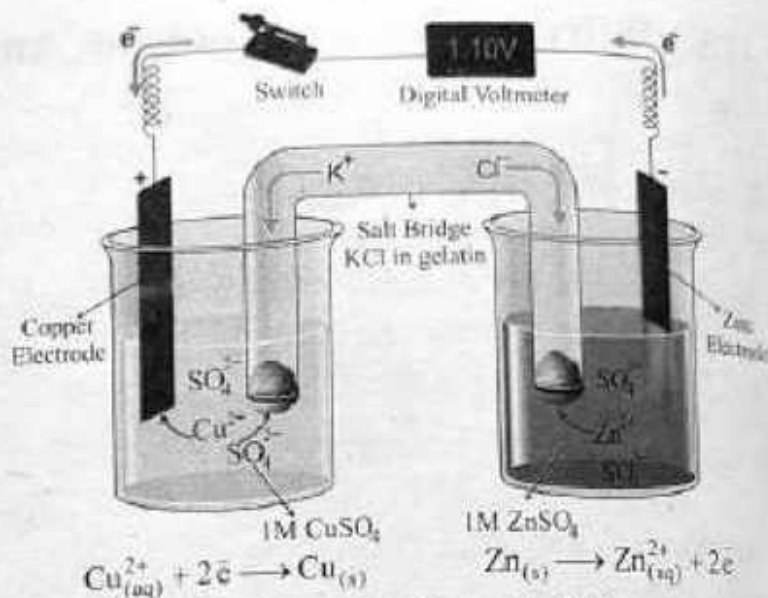
Figure 12.3: Galvanic Cell
