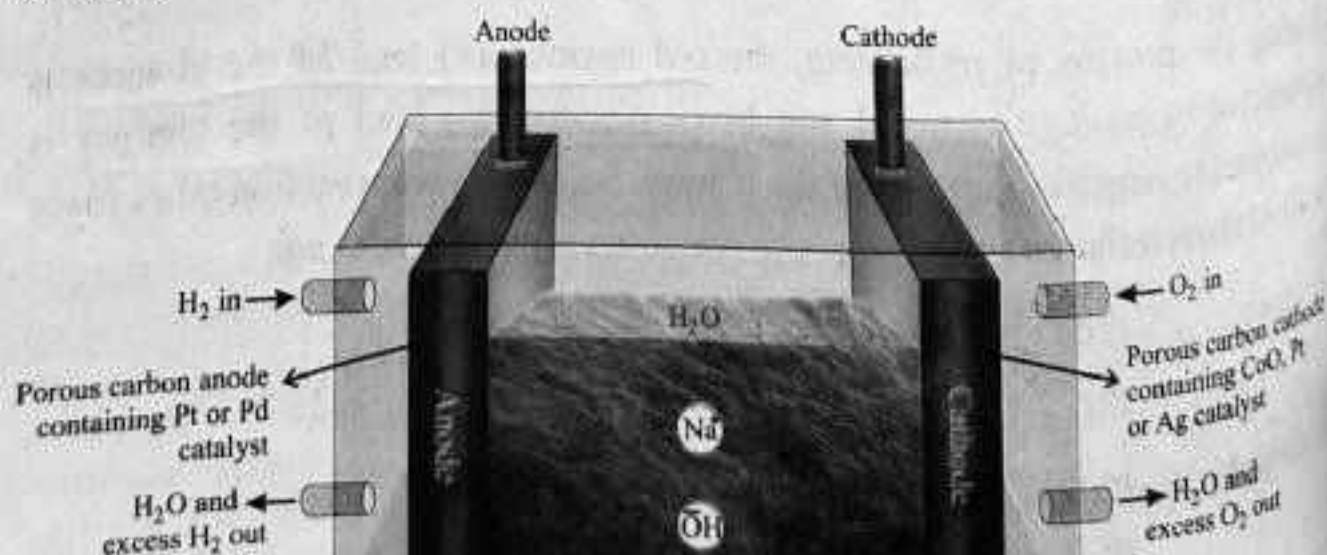
Figure 12.9: Fuel Cell
