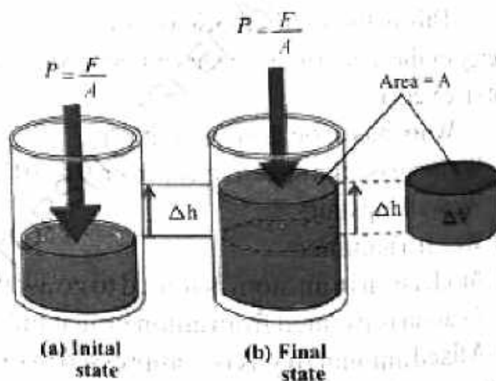
Figure 11.1: Pressure-volume Work
