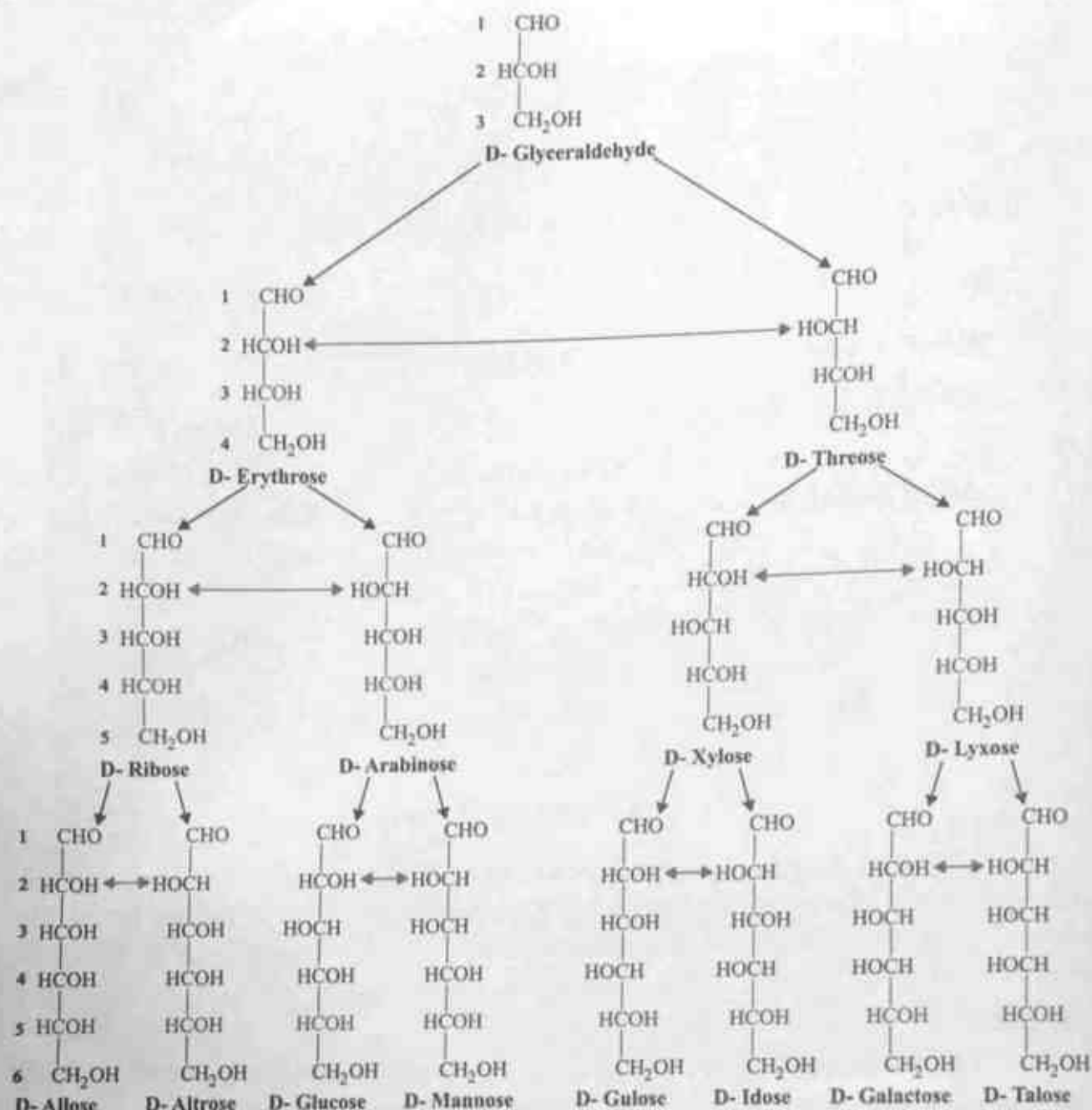
Fig. 2.5(a) Stereochemistry of the D-aldoses
