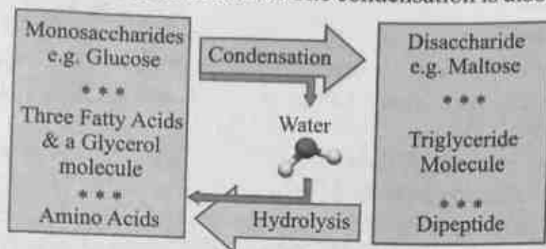
Fig. 2.1 Condensation and Hydrolysis
