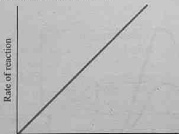
Fig. 3.7 Enzyme Concentration
