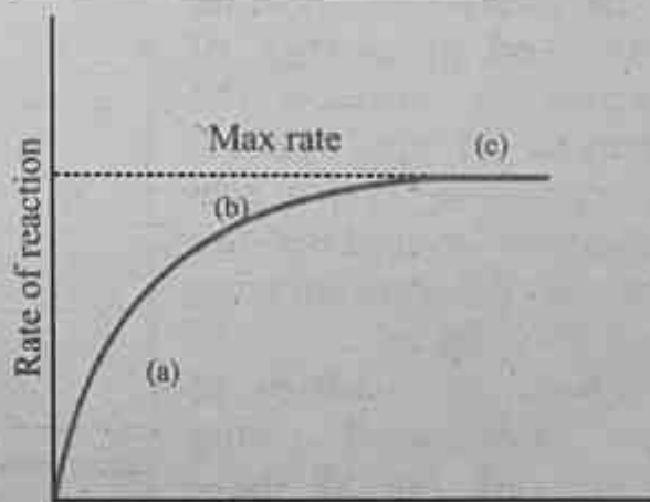
Fig. 3.8 Concentration of Substrate
