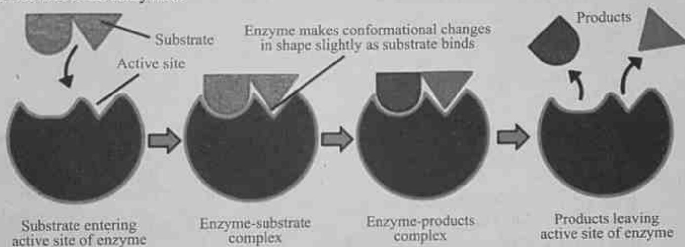
Fig.3.1 Mechanism of Enzyme Action
