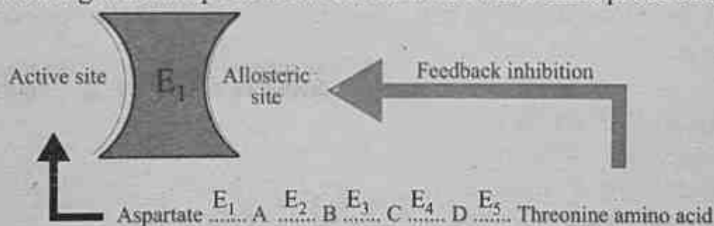
Fig. 3.11 Feedback Inhibition
