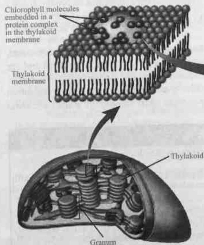
Fig. 4.1 Structure of chloroplast and chlorophyll
