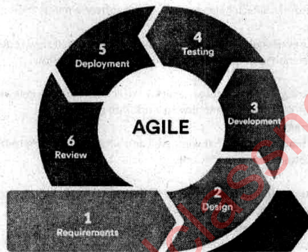
Figure 1.3: Agile Methodology
