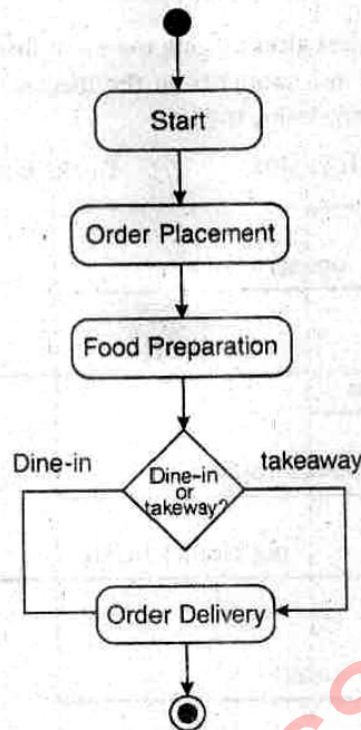
Figure 1.12: Activity Diagram with Decision and Connector Symbol
