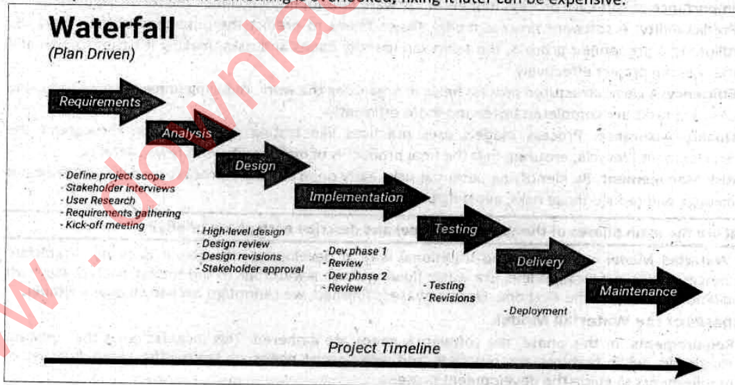
Figure 1.2: Waterfall Model
