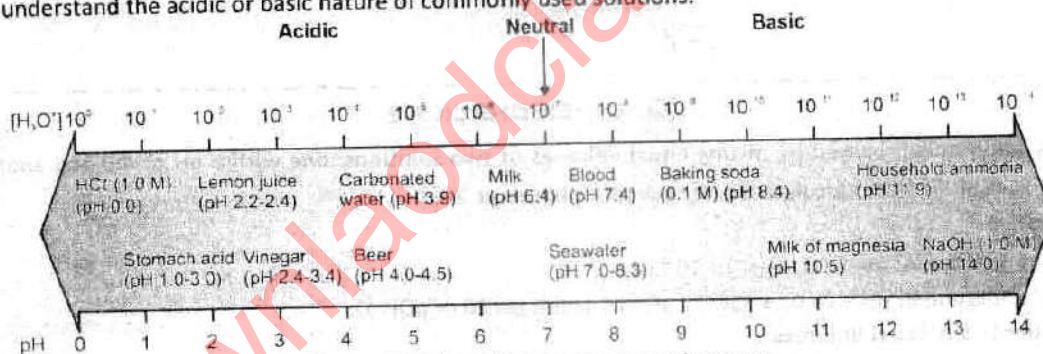
Figure: pH Values of some common substances
