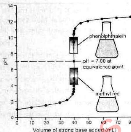
Figure: Strong acid-strong base titration curve
