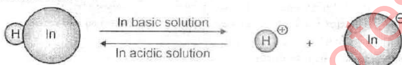
Figure: Unionized acid-base indicators and their ionised forms exist in an equilibrium
