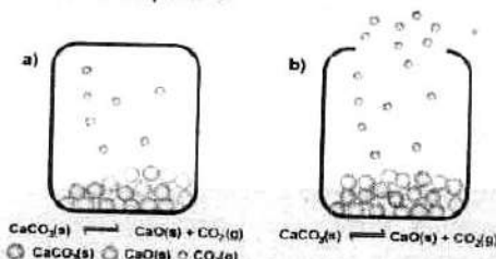
Figure (a): Equilibrium is established when the system is closed (b) Equilibrium cannot be established in the open system.
