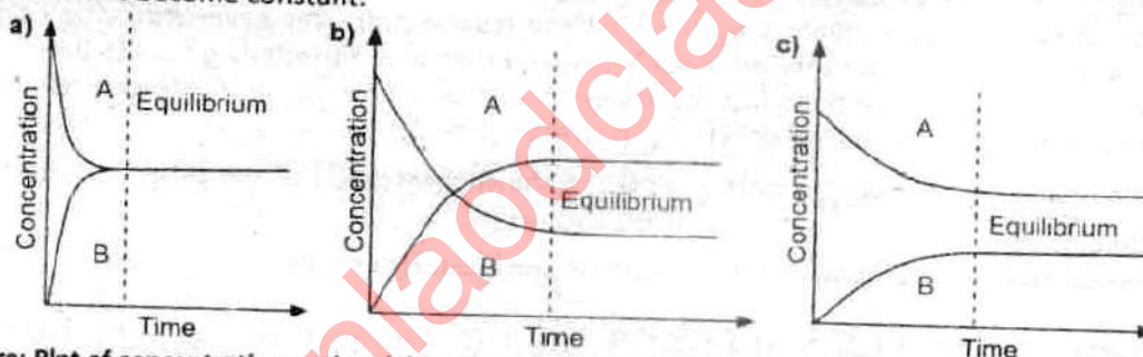
Figure: Plot of concentration vs time (a) Reactant = Product (b) Reactant < Product (c) Reactant > Product
