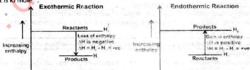
Enthalpy changes in thermochemical reactions
