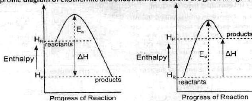
Figure: Energy profile diagram in terms of \Delta H and E_a
