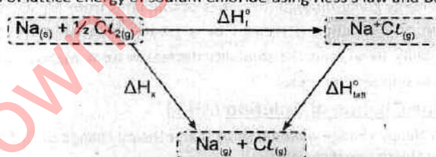
Figure: Enthalpy cycle of sodium chloride
