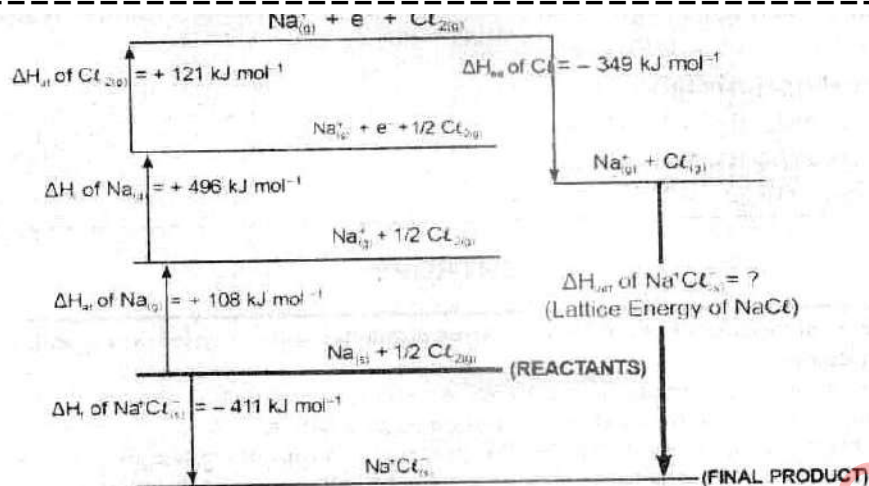
Figure: Born-Haber cycle of sodium chloride (not according to scale)
