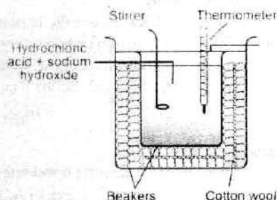
Figure: Glass calorimeter to measure enthalpy change of reactions
