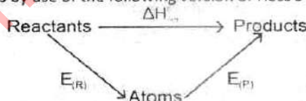
Figure: Hess Cycle; showing the relationship between B.E.'s and \Delta H_r = \sum nE_R - \sum nE_P
