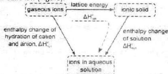
Figure: Energy cycle of formation of an aqueous solution of an ionic solid using Hess's law
