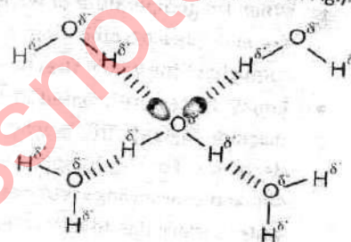
Figure: Hydrogen bonding in water
