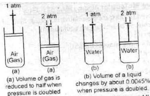
Figure: Effect of pressure on the volumes of gases and liquids.
