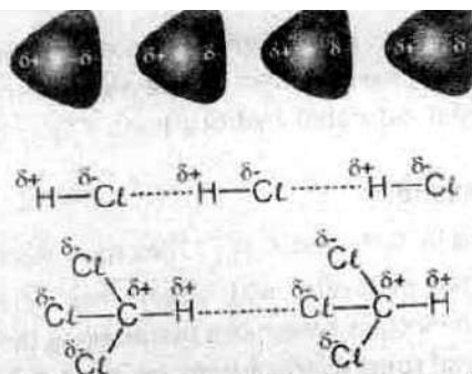
Figure: Permanent dipole-permanent dipole forces in HCl and chloroform
