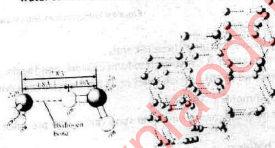
Figure: Extensive hydrogen bonding in ice and spaces among molecules
