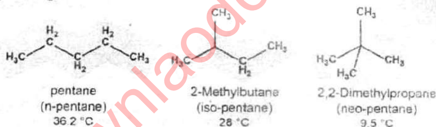
Figure: The three isomers of pentane have different structures, surface areas and intermolecular forces
