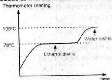
Figure: Fractional distillation of ethanol / water mixture
