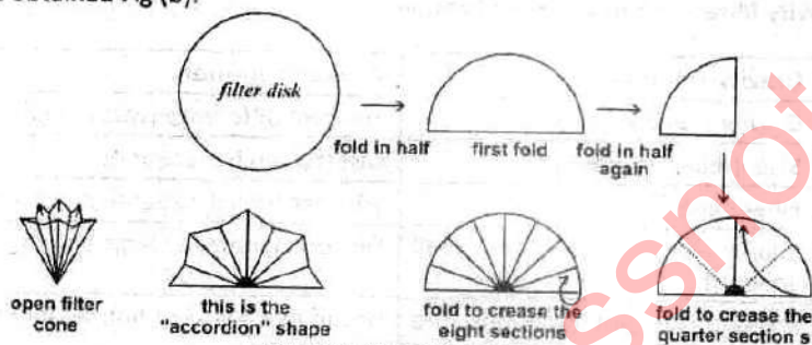
Figure b: Fluted filter paper
