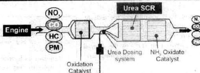
Figure: Selective Catalytic Reduction
