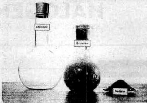
Figure: The greenish yellow chlorine (left), orange bromine (middle) and purple iodine (right)
