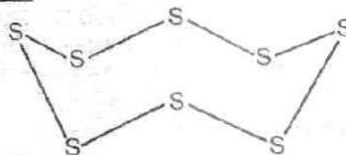
Figure: Cyclo-octasulphur, ( S_8 ) crown molecule
