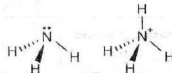
Figure: Pyramidal and tetrahedral shapes of ammonia and ammonium
