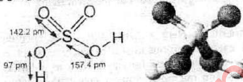
Figure: Structure of H 2 SO 4
