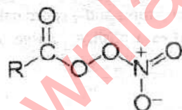
Figure: General structure of PANs
