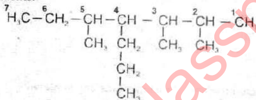
2, 3, 5 - Trimethyl - 4 - n - propylheptane
