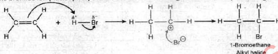
Figure: Electrophilic addition mechanism of HBr to ethene
