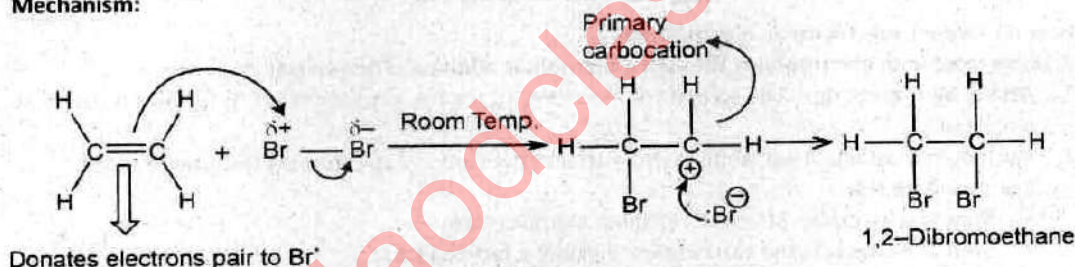
Figure: Electrophilic addition mechanism of ethene and \text{Br}_2
