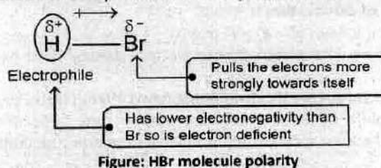
Figure: \text{HBr} molecule polarity
