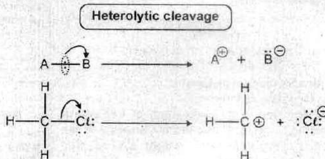
Figure: Heterolytic fission and formation of radical ions
