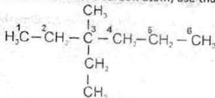
3 - Ethyl - 3 - methylhexane
