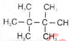
2, 2, 3, 3 - Tetramethylbutane
