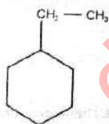
Ethylcyclohexane
