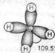
Methane sp^3 hybrid tetrahedral
