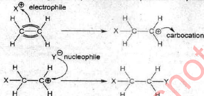
Figure: Generalized mechanism of electrophilic addition
