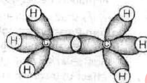
Ethane
