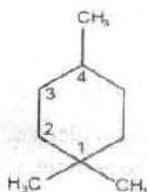
1,1,4-Trimethylcyclohexane
