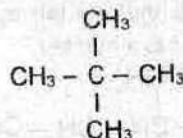
2,2-Dimethylpropane
