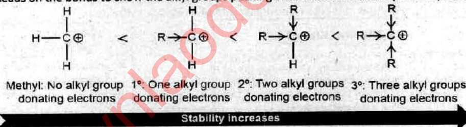
Figure: Inductive effect & stability of carbocation
