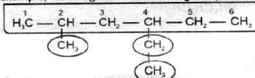
4-Ethyl-2-methylhexane
