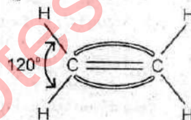
Figure: Structure of ethene
