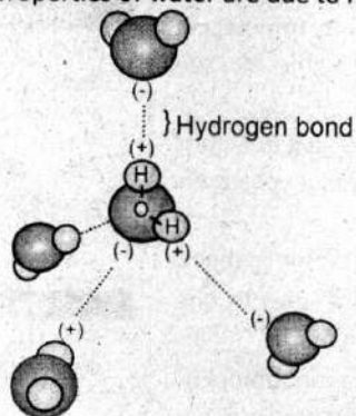
Figure: Hydrogen bonds among water molecules
