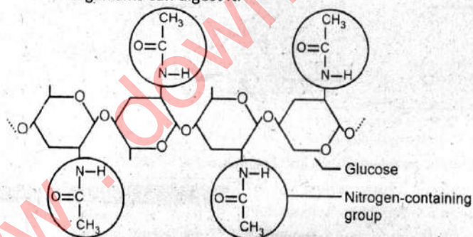
Figure: A part of the chitin molecule
