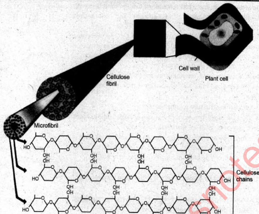
Figure: Cellulose fibrils in plant cell wall
