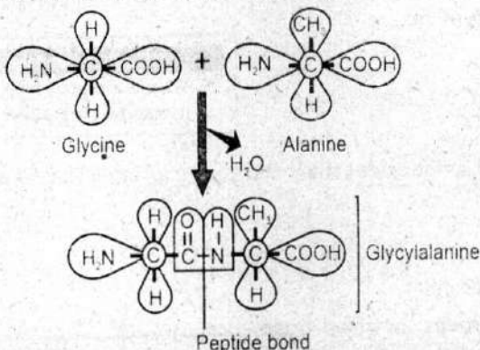
Figure: Formation of peptide bond between glycine and alanine
