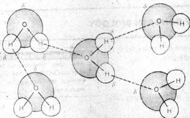
Figure: Hydrogen bond between water molecules
