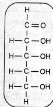
Figure: Structure of Ribose
