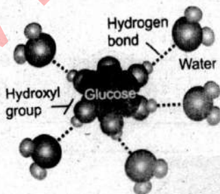
Figure: Water as a solvent of organic molecules (glucose)
