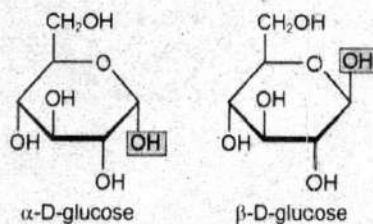
Figure: Ring structures of glucose, galactose, fructose, and ribose
