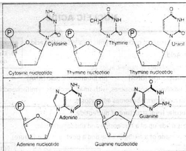
Figure: Nucleotides of RNA and DNA
