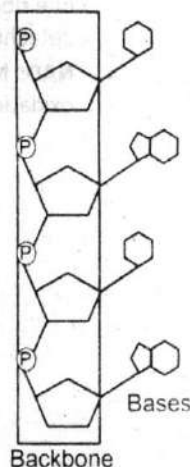
Figure: Sugar-phosphate backbone of nucleic acids
