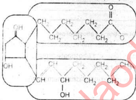
Figure: A prostaglandin
