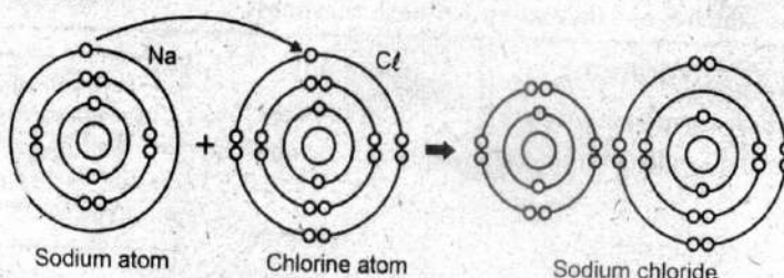
Figure: Ionic bond between sodium and chlorine atoms
