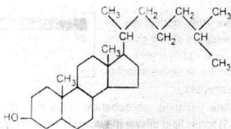
Figure: Cholesterol: a steroid
