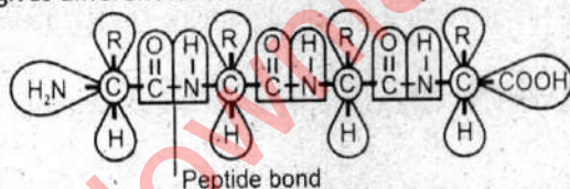
Figure: Section from a polypeptide chain
