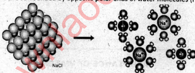
Figure: Water as a solvent of inorganic molecules (NaCl)
