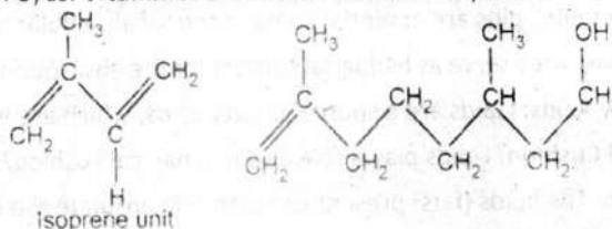
Figure: Structure of terpenes
