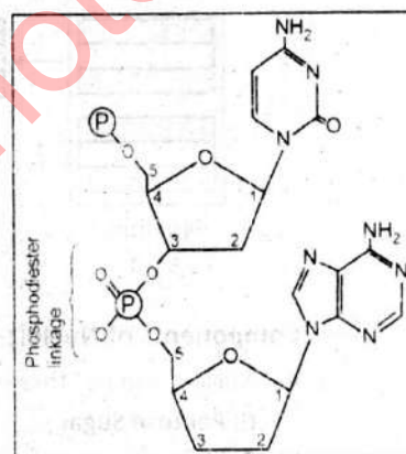
Figure: A dinucleotide
