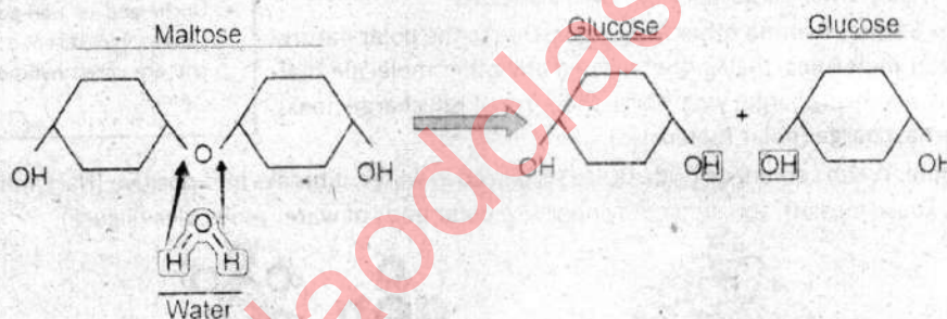
Figure: Breaking of macromolecules (Hydrolysis)
