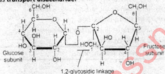
Figure : Structure of sucrose
