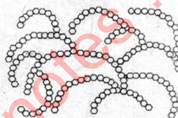
Figure: (a) amylose, (b) amylopectin
