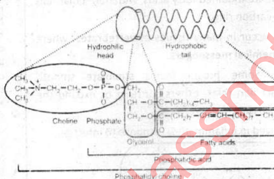
Figure: Phosphatidyl choline – a phospholipid
