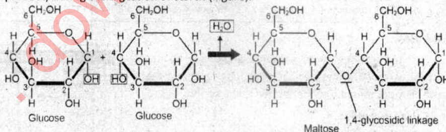
Figure: Dehydration synthesis of one maltose by the condensation of two glucose
