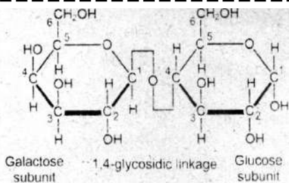
Figure : Structure of lactose
