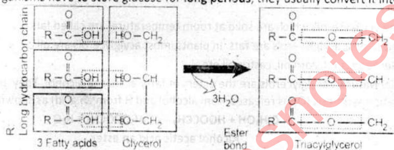
Figure: Dehydration synthesis of a triacylglycerol
