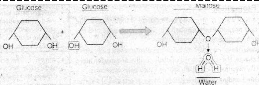
Figure: Making of macromolecules (Dehydration synthesis)
