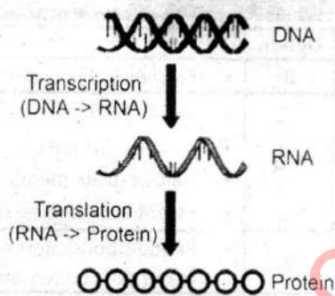
Figure: Flow sheet of Central dogma
