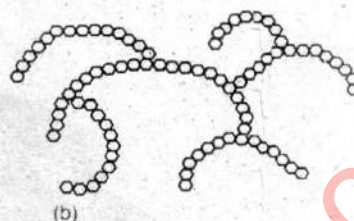
Figure: (a) amylose, (b) amylopectin
