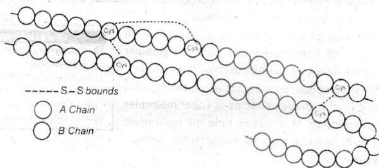
Figure: Chains of Insulin
