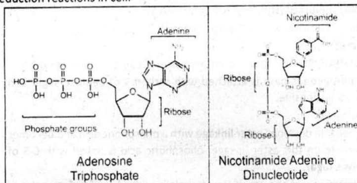
Figure: ATP and NAD
