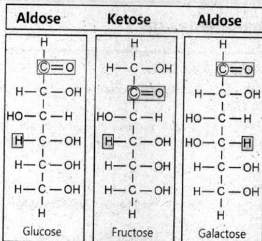
Figure: Structural and stereoisomers of glucose
