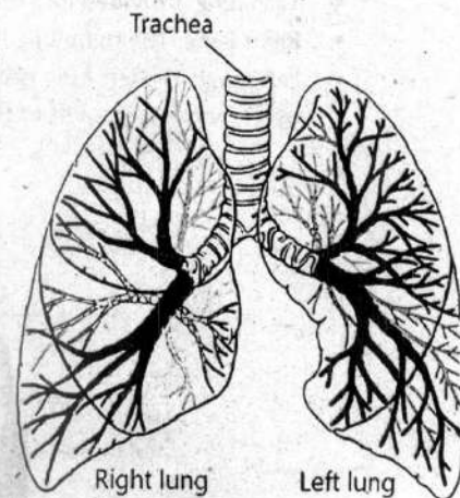
Figure: Tree-like branching of the lower respiratory tract
