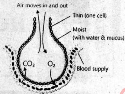
Figure: Some properties of respiratory surface
