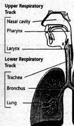
Figure: Respiratory track
