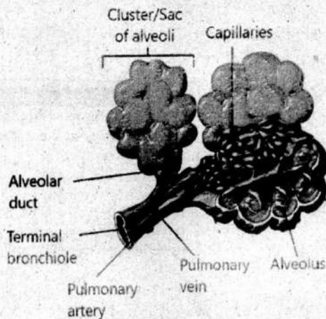
Figure: Clusters of alveoli
