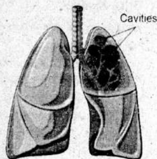
Figure: A lung affected with TB
