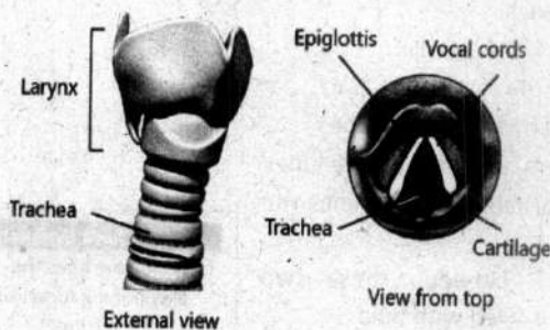
Figure: Larynx and Trachea
